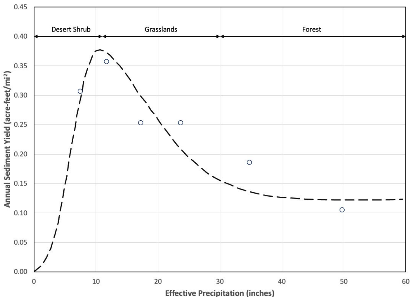
Figure 8.3. Annual sediment yield as a function of effective mean annual precipitation and associated vegetation types (replotted from original by Langbein and Schumm, 1958).
