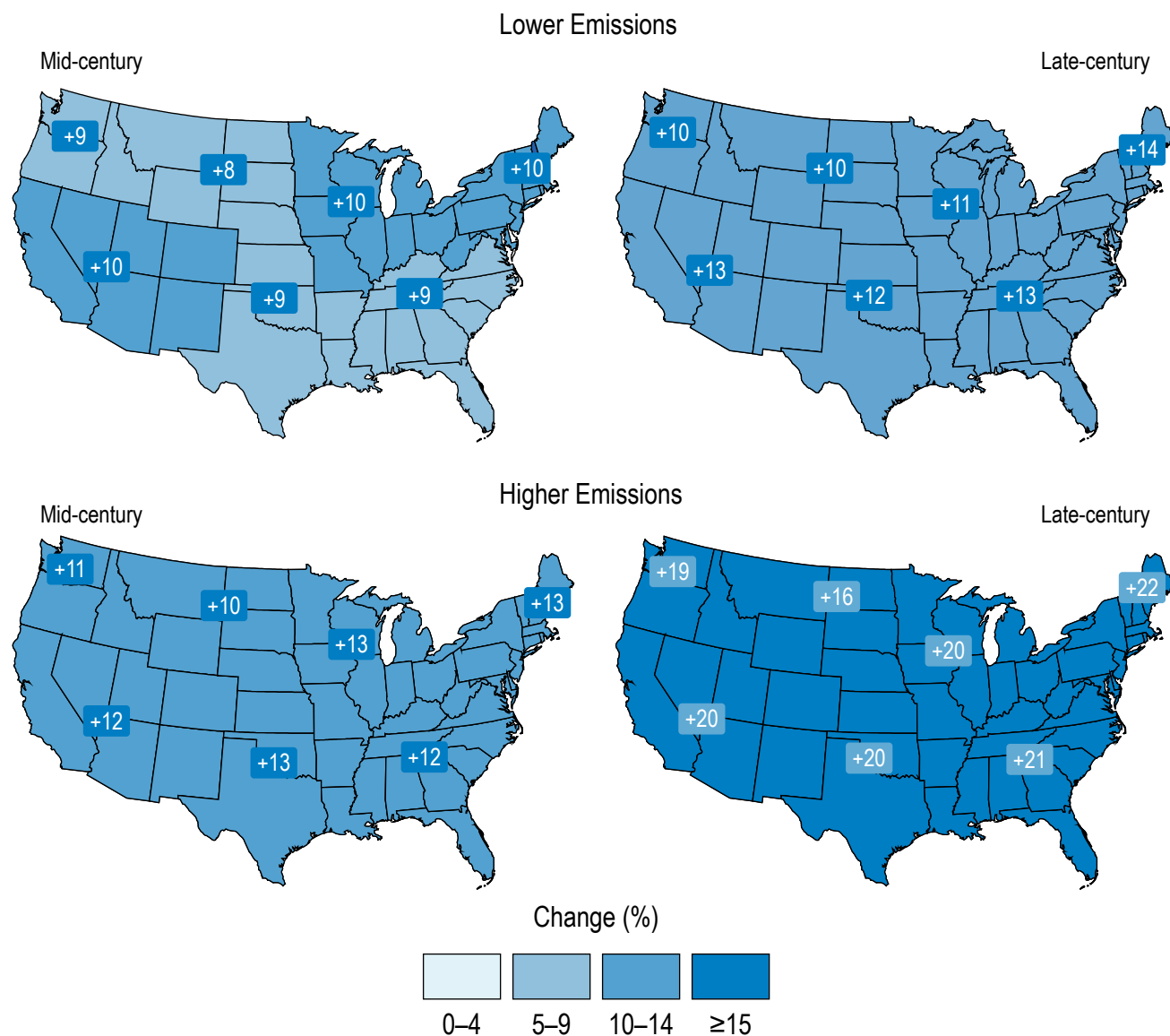
Figure 2.5. Projected change from a historical baseline period (1901–2005) in the magnitude of extreme precipitation events, here defined as the 1-day precipitation maximum expected once every 20 years, derived from statistically downscaled CMIP5 global climate model simulations (using an average of CMIP5 models but a different statistical downscaling technique than the MACA post-processing used for Figures 2.1–2.4; USGCRP, 2017, Figure 7.7). Results from a lower emissions scenario (RCP 4.5) are on the top; higher scenario results (RCP 8.5) are on the bottom. The left-side maps show changes as a percentage of present-day 20-year return values expected by mid-century; late-twenty-first-century changes are shown on the right. All changes projected nationwide are positive, indicative of higher 20-year return values of maximum daily precipitation.
