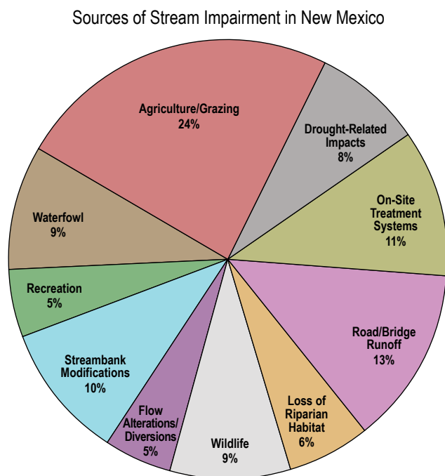
Figure 10.4. Probable sources of surface-water impairment in streams and rivers of New Mexico, as reported in approved TMDLs (NMED, 2021a).
