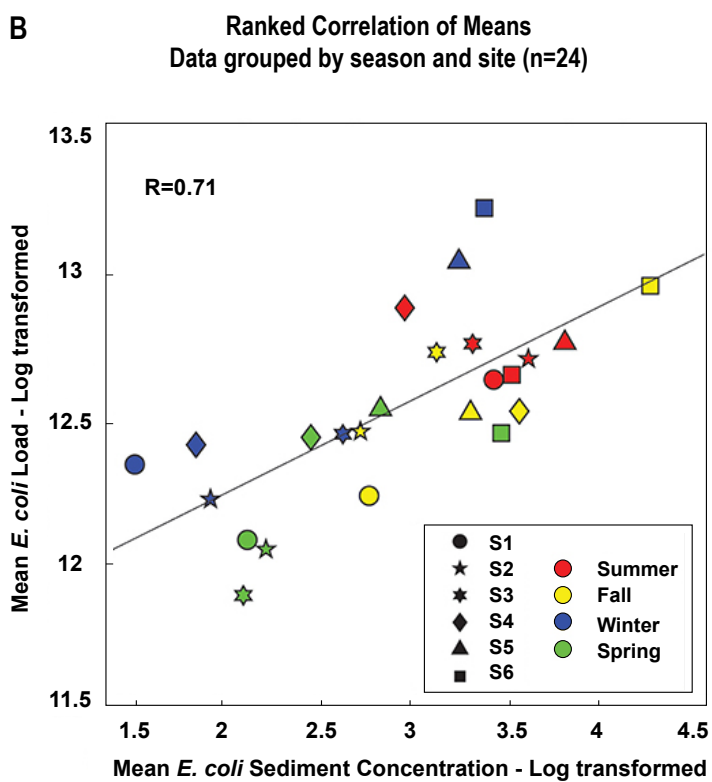
Figure 10.9. (A) Correlation between E. coli water and sediment concentrations and (B) E. coli water loads and mean E. coli sediment concentrations in stream bottom sediments in the Middle Rio Grande. Sites are numbered from the upstream extent of the watershed (site S1) to the downstream extent (site S6; Fluke et al., 2019).
