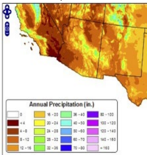
Figure 1.1. 30-year average “normal” values of observed mean annual temperature (A) and observed mean annual precipitation (B) from 1981 to 2010. From PRISM group at Oregon State University in 2021.
