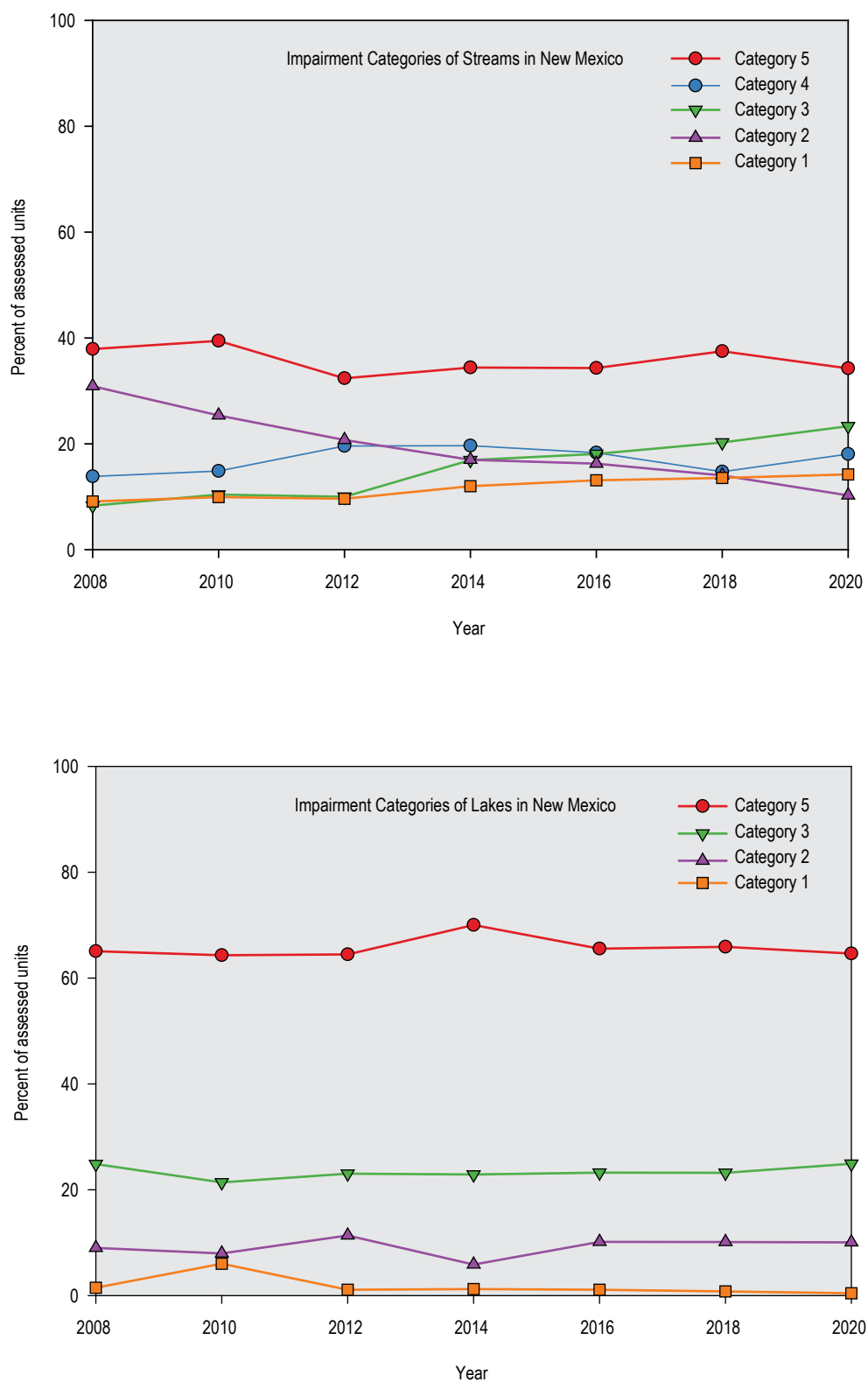
Figure 10.1. Summary of the impairment categories of assessed streams and lakes in New Mexico (NMED, 2021a). A description of the assessment categories is provided in Table 10.2.
