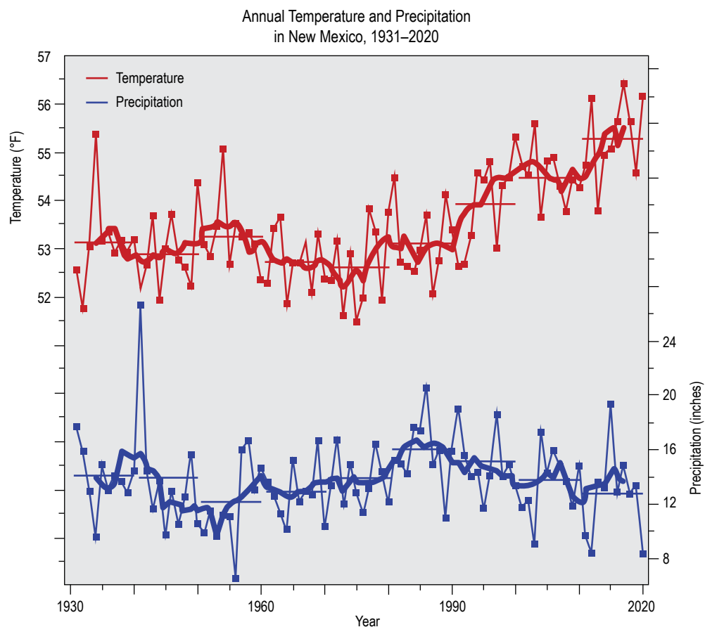
Figure 1.2. Observed annual temperature (red) and precipitation (blue) averaged over the state of New Mexico, 1931–2020. Horizontal lines depict 10-year decadal averages for each calendar decade. Updated from Chermak et al. (2015) and Gutzler (2020).
