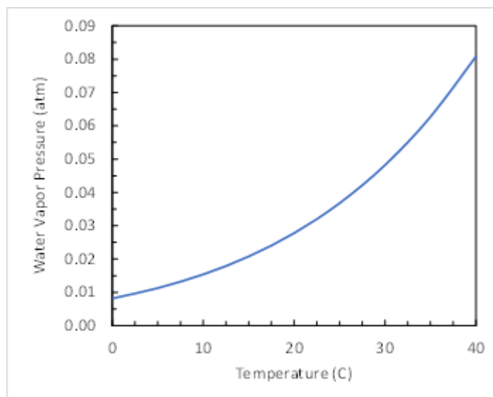
Figure C.1. Relationship between saturation water vapor pressure (over a flat surface of liquid water) and air temperature.
