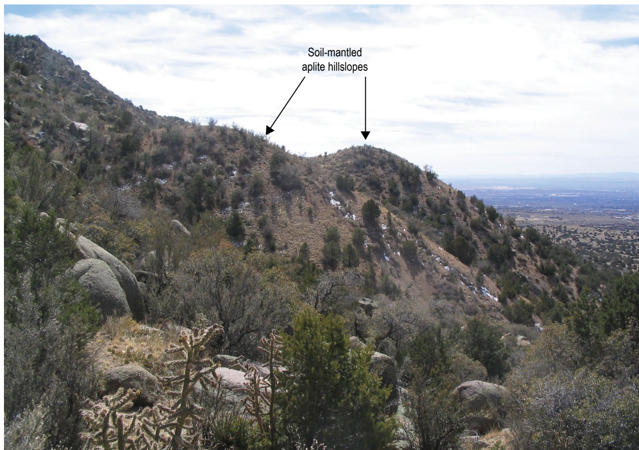
Figure 5.6. Core-stone-dominated hillslopes (in left foreground) are the dominant kind of hillslope in the Sandia Mountains foothills formed on granitic rocks. Two smooth, soil-mantled, transport-limited hillslopes are labeled. Understanding how such soils and hillslopes form provides the basis for predicting how they have responded to past climate changes and how they may respond to the next 50 years of climate change.
